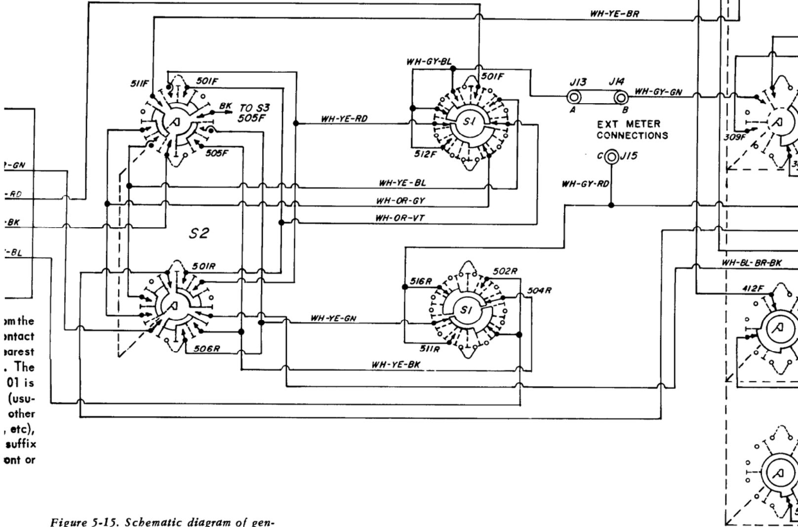
Figure 5-15. Schematic diagram of generator and detector switching.
