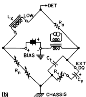
Figure 3-2. Methods of applying dc to inductors.
