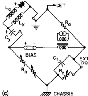
Figure 3-2. Methods of applying dc to inductors.
